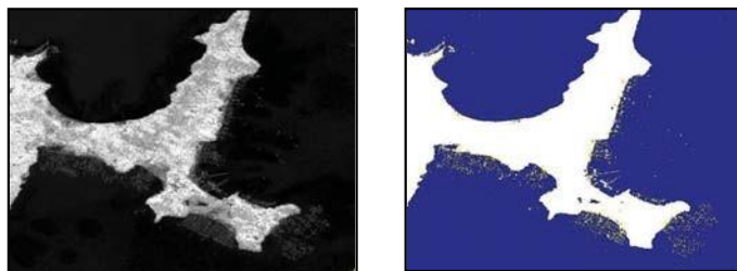
Figure 4: Band ratio of NIR/Green band (760-900/630-690)
